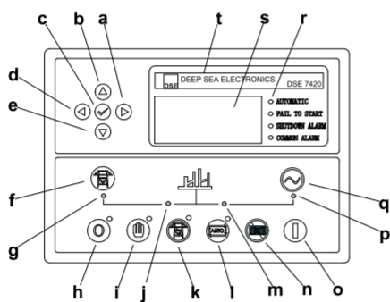
Control module
